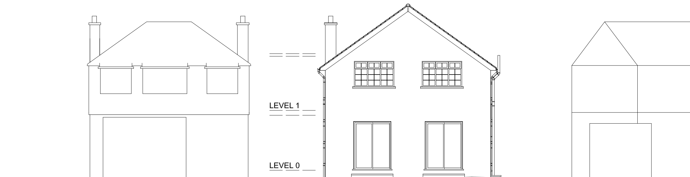
REAR ELEVATION
